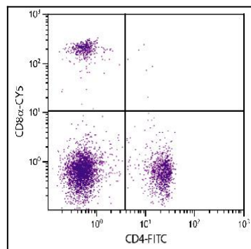
Figure 1: BALB/c mouse splenocytes were stained with Rat Anti-Mouse CD8a-CY5 and Rat Anti-Mouse CD4-FITC .
