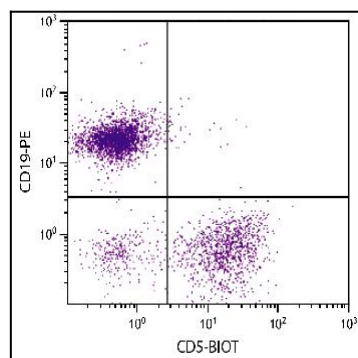
Figure 1: BALB/c mouse splenocytes were stained with Rat Anti-Mouse CD5-Biotin and Rat Anti-Mouse CD19-PE followed by Streptavidin-FITC .
