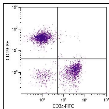
Figure 1: BALB/c mouse splenocytes were stained with Hamster Anti-Mouse CD3e-FITC and Rat Anti-Mouse CD19-PE .
