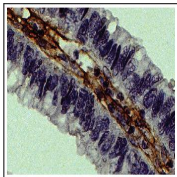
Figure 1: Human gastric cancer tissue was stained with Goat Anti-Type III Collagen followed by Swine Anti-Goat IgG(H+L), Human/Rat/Mouse SP ads-HRP .
