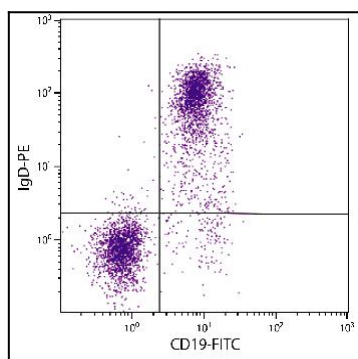
Figure 1: BALB/c mouse splenocytes were stained with Rat Anti-Mouse IgD-PE and Rat Anti-Mouse CD19-FITC .
