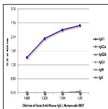
Figure 1: ELISA plate was coated with purified mouse IgG1, IgG2a, IgG2b, IgG3, IgM, and IgA. Immunoglobulins were detected with serially diluted Goat Anti-Mouse IgG1, Human ads-Biotin followed by Streptavidin-HRP .
