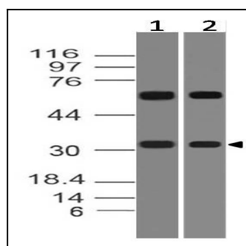
Fig-1: Western blot analysis of HoxD8. Anti-HoxD8 antibody (11-12047) was used at 2 µg/ml on(1) A375 and (2) NCCIT lysates.
