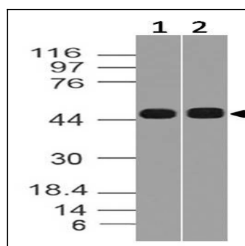
Fig-1: Western blot analysis of SOX17. Anti- SOX17 antibody (11-12010) was used at 4 µg/ml on (1) HepG2 and (2) HCT-116 lysates.
