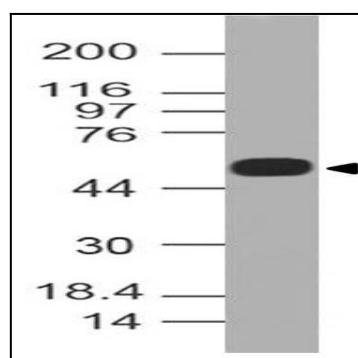
Fig-1: Western blot analysis of AIRE/APECED. Anti-AIRE/APECED antibody (11-4010) was used at 1 µg/ml on h Liver lysate.
